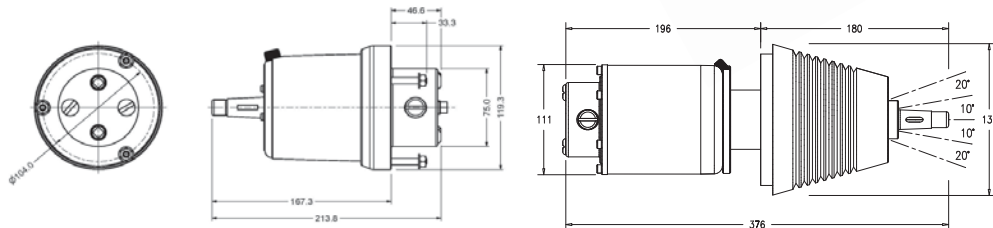
Fully tilting helm design Model 101 - Tilt or 102 - Tilt
