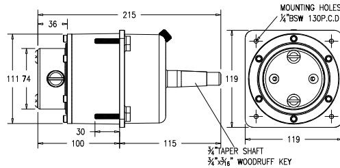
OPTIONAL Model 101 & 102 Mid-mount helm unit
