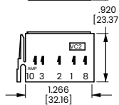
VC2 CONNECTOR HOUSING (For AMP terminals only)
