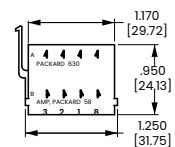
VCH CONNECTOR HOUSING
