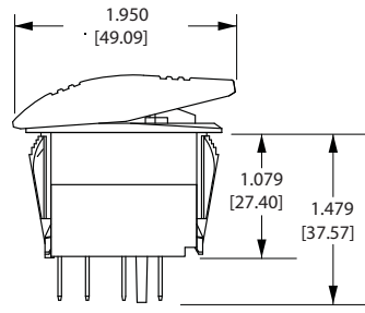
8 TERMINAL BASE W/O BARRIERS
