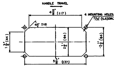
"OUT-OUT" DIMENSIONS
